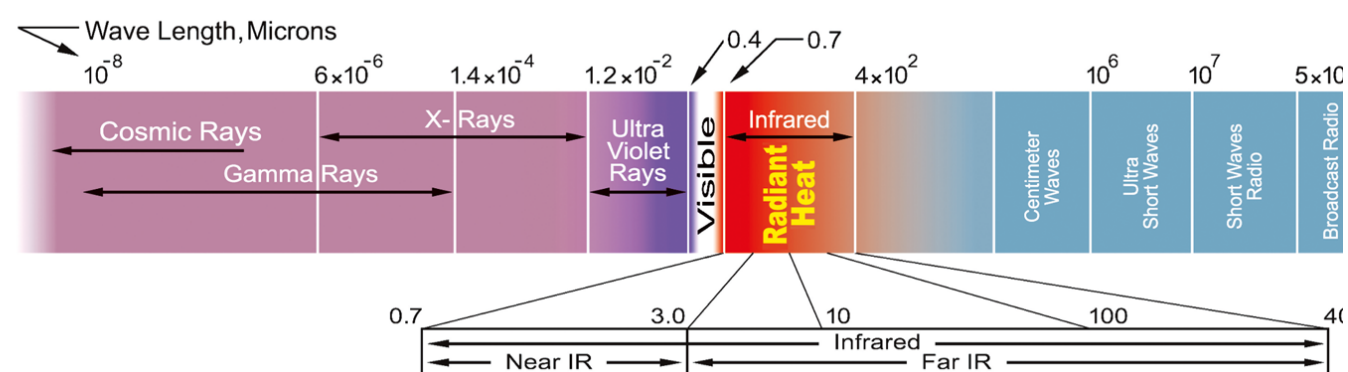
Electromagnetic spectrum
